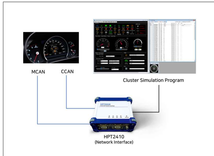
통합형 Cluster CAN Simulator
