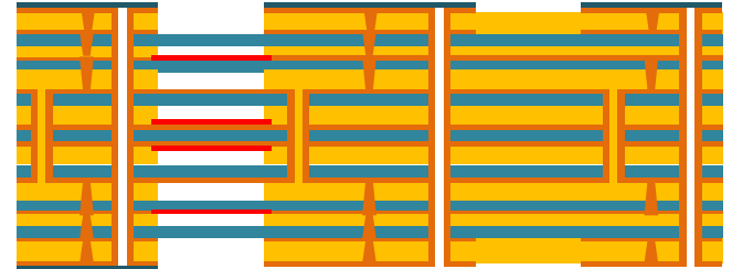
Rigid Flexible PCB
